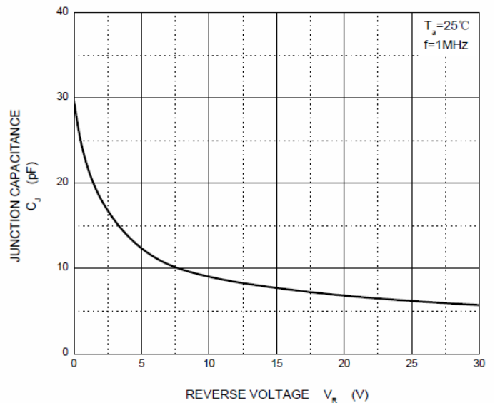
Capacitance Characteristics
