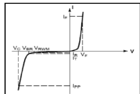
V-I characteristics for a uni-directional TVS
