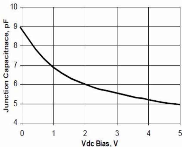
Off-State Capacitance vs DC Bias
