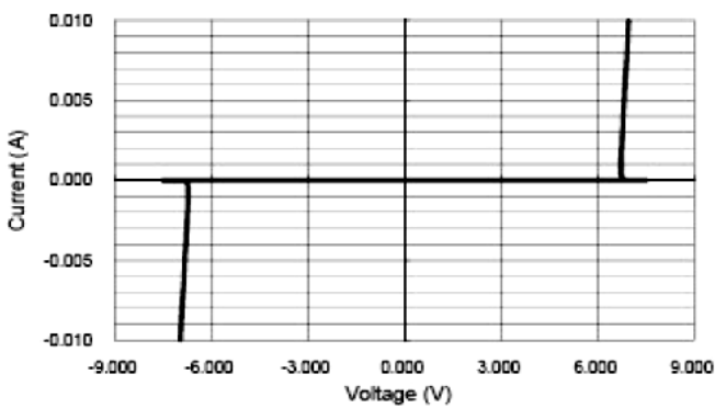
Fig 3 Voltage Sweeping
